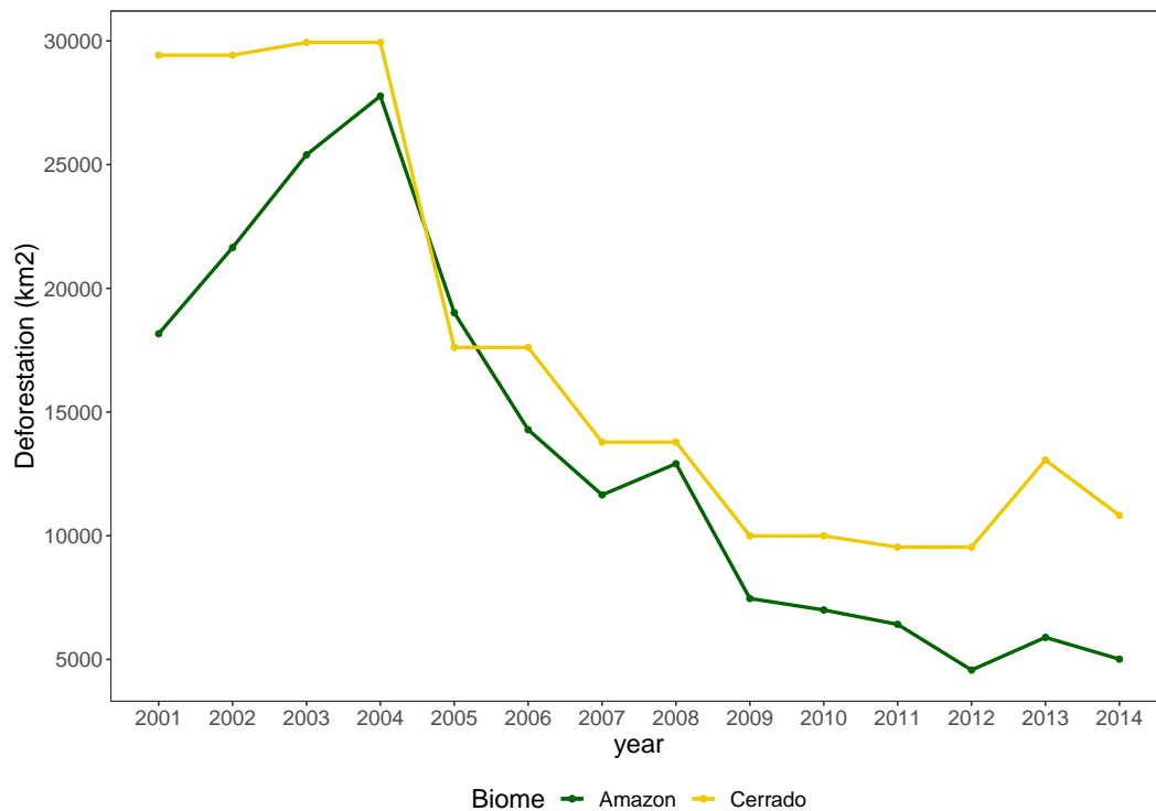
Figure 2: Deforestation Trends (2001 - 2014)
